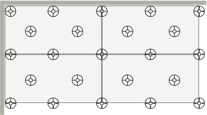
Posa sopraelevata 60×120 \pm 2 cm 24"x48" \pm ¾" Installation onto flat surfaces (raised laying)
