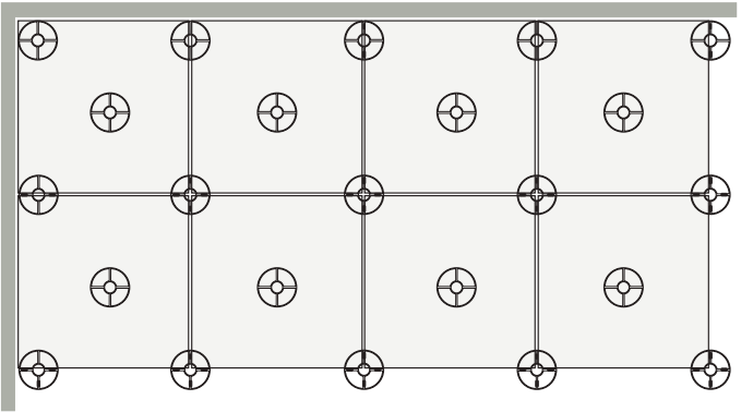
Posa sopraelevata 60×60 \pm 2 cm 24"x24" \pm ¾" Installation onto flat surfaces (raised laying)
